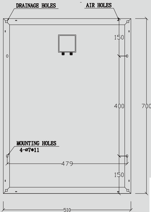
Engineering Drawings (Back Side)
